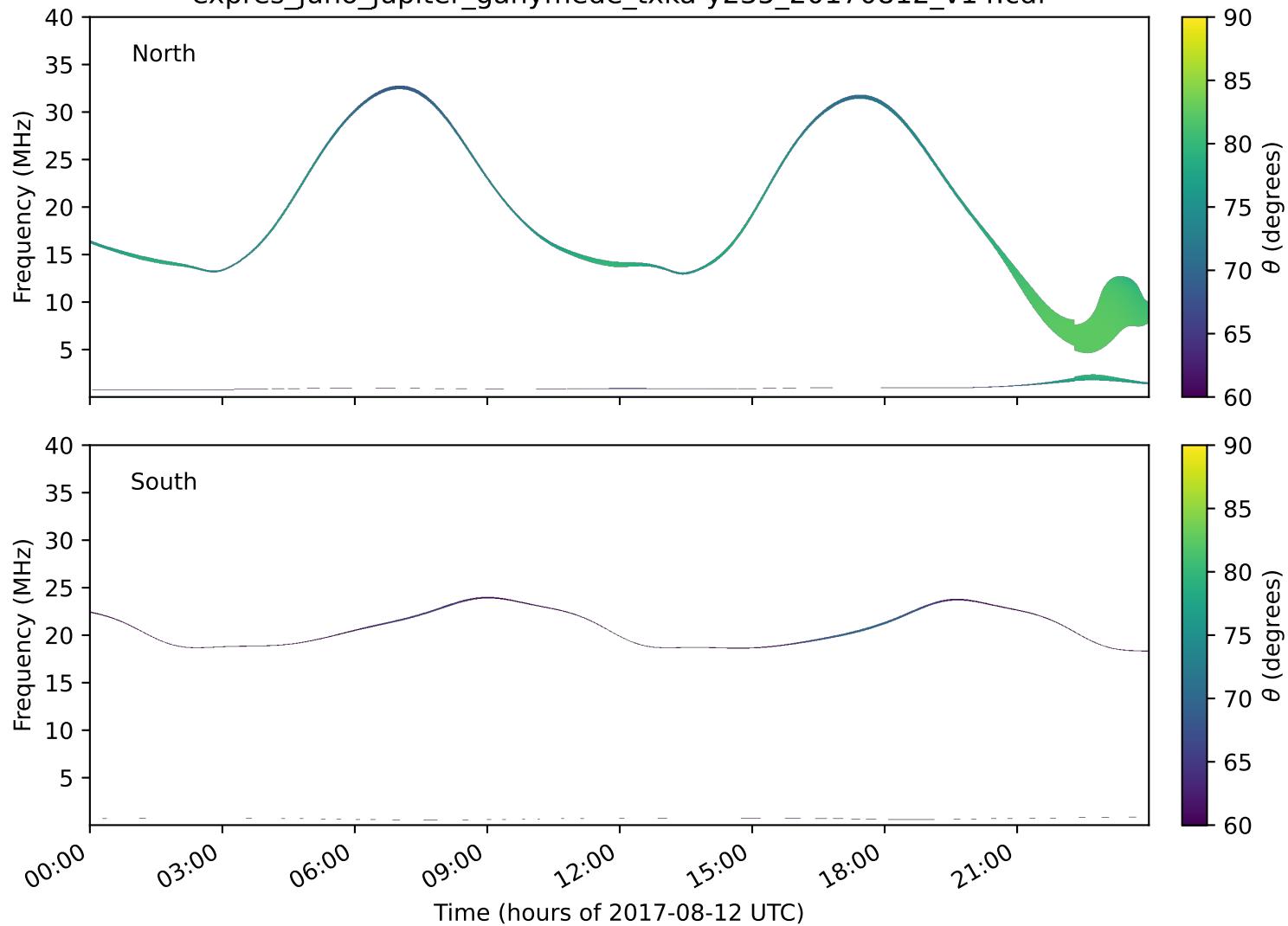
expres_juno_jupiter_ganymede_txka-y235_20170812_v14.cdf
