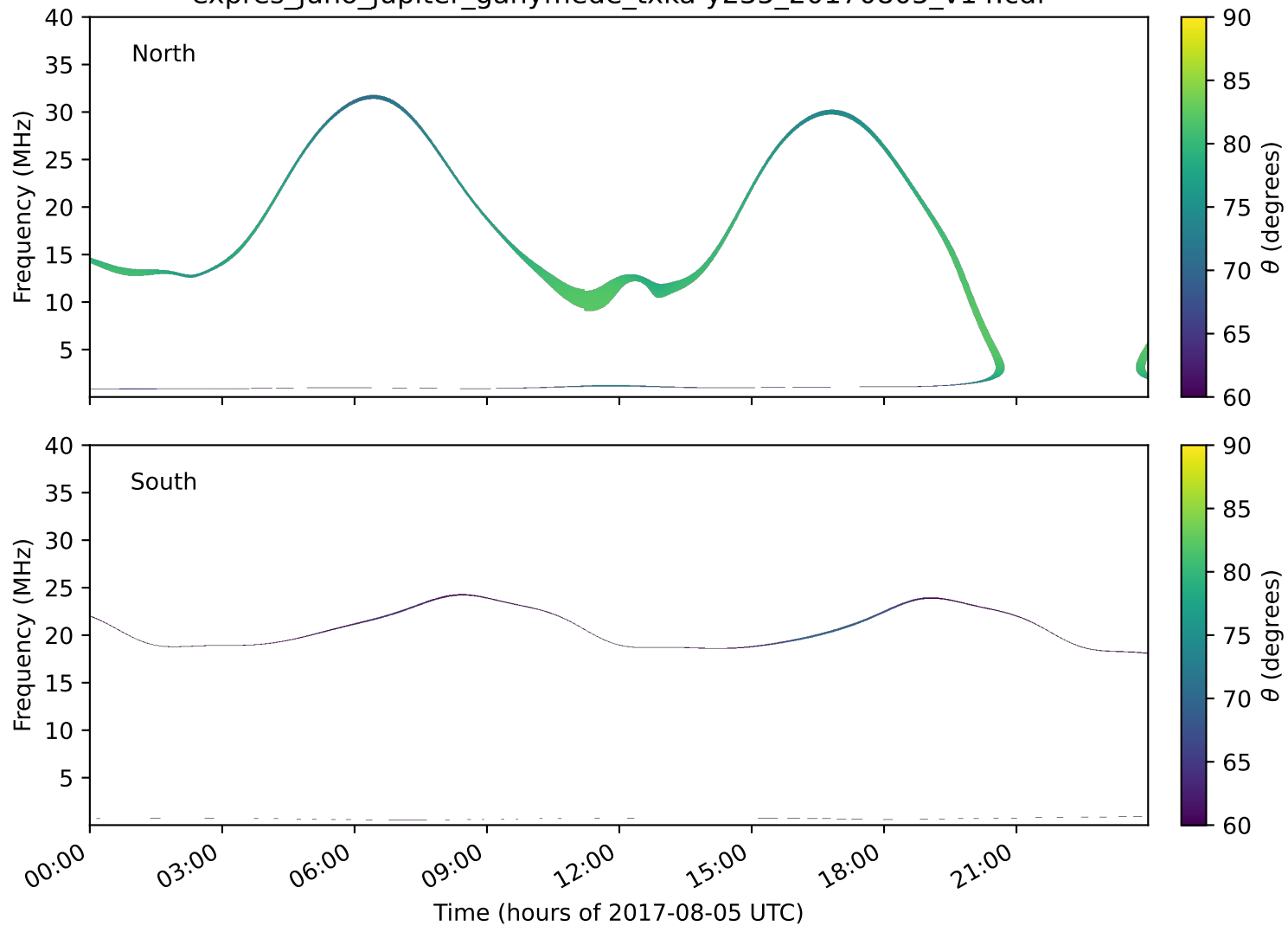
expres_juno_jupiter_ganymede_txka-y235_20170805_v14.cdf
