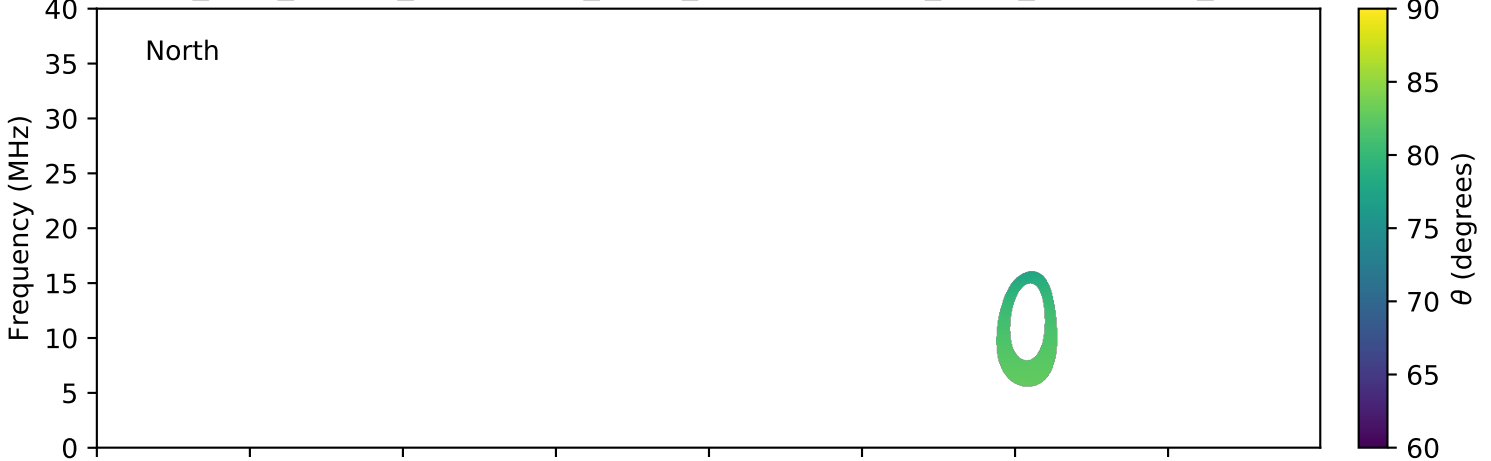
expres_juno_jupiter_ganymede_isaac_lossc-wid1deg_3kev_20170831_v01.cdf
