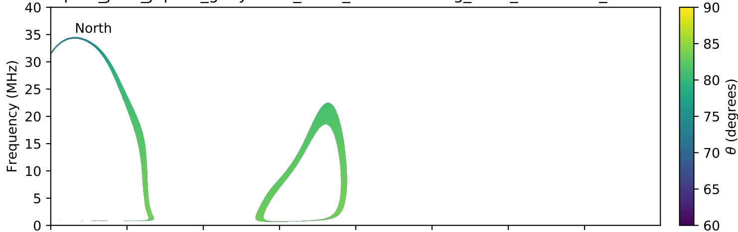
expres_juno_jupiter_ganymede_isaac_lossc-wid1deg_3kev_20170828_v01.cdf
