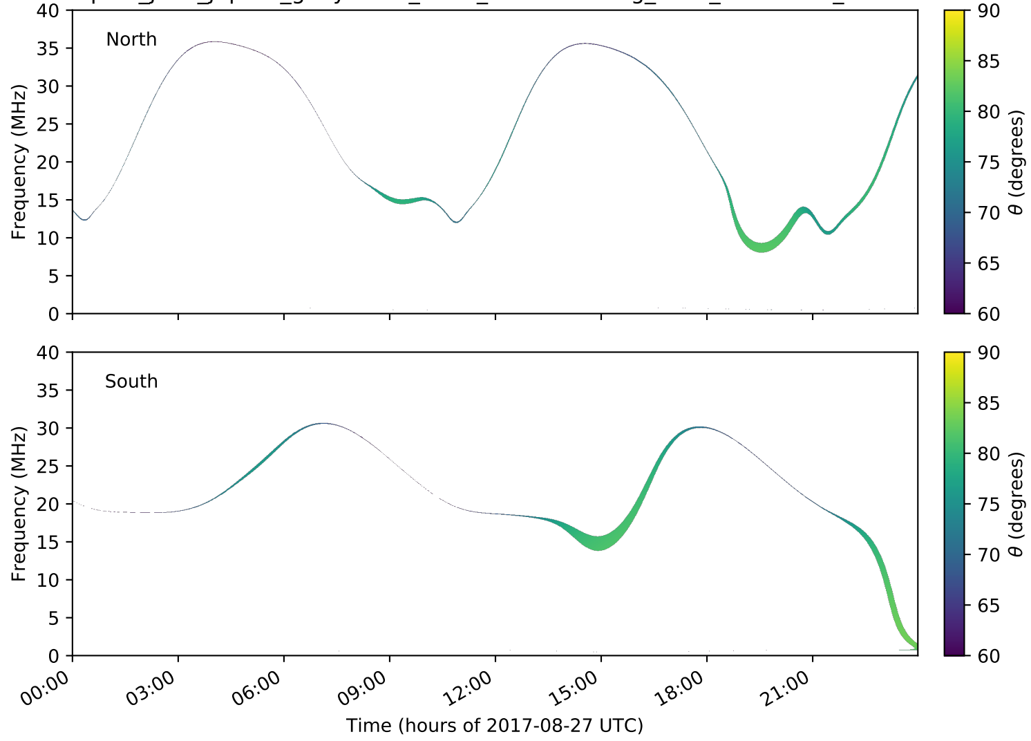
expres_juno_jupiter_ganymede_isaac_lossc-wid1deg_3kev_20170827_v01.cdf
