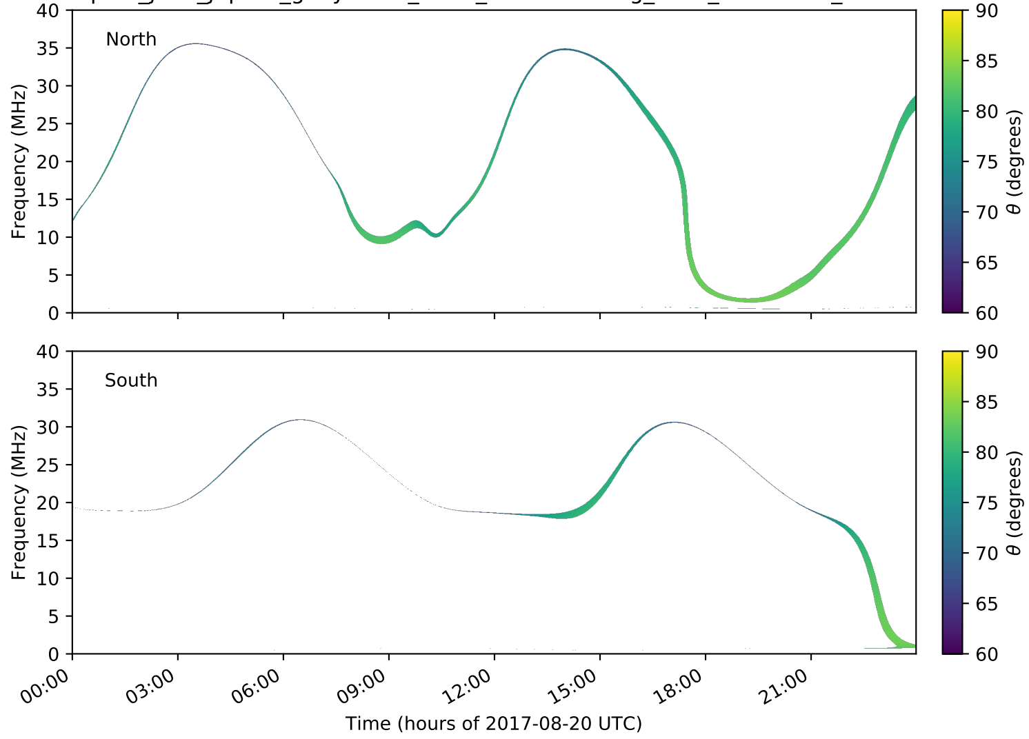
expres_juno_jupiter_ganymede_isaac_lossc-wid1deg_3kev_20170820_v01.cdf
