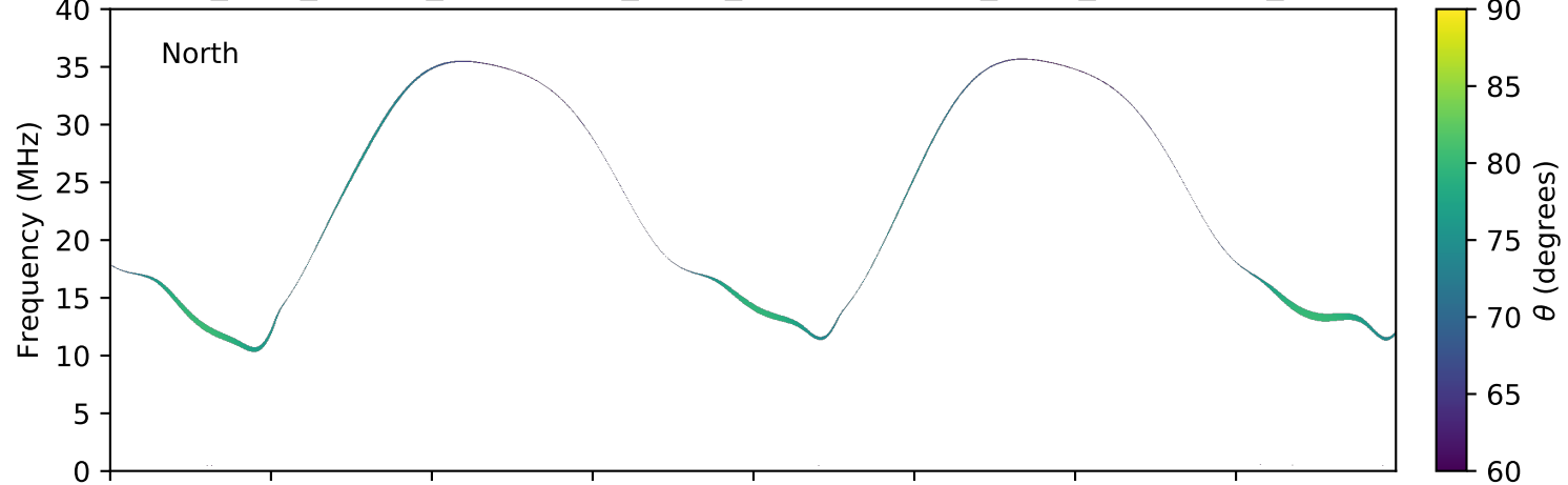
expres_juno_jupiter_ganymede_isaac_lossc-wid1deg_3kev_20170819_v01.cdf
