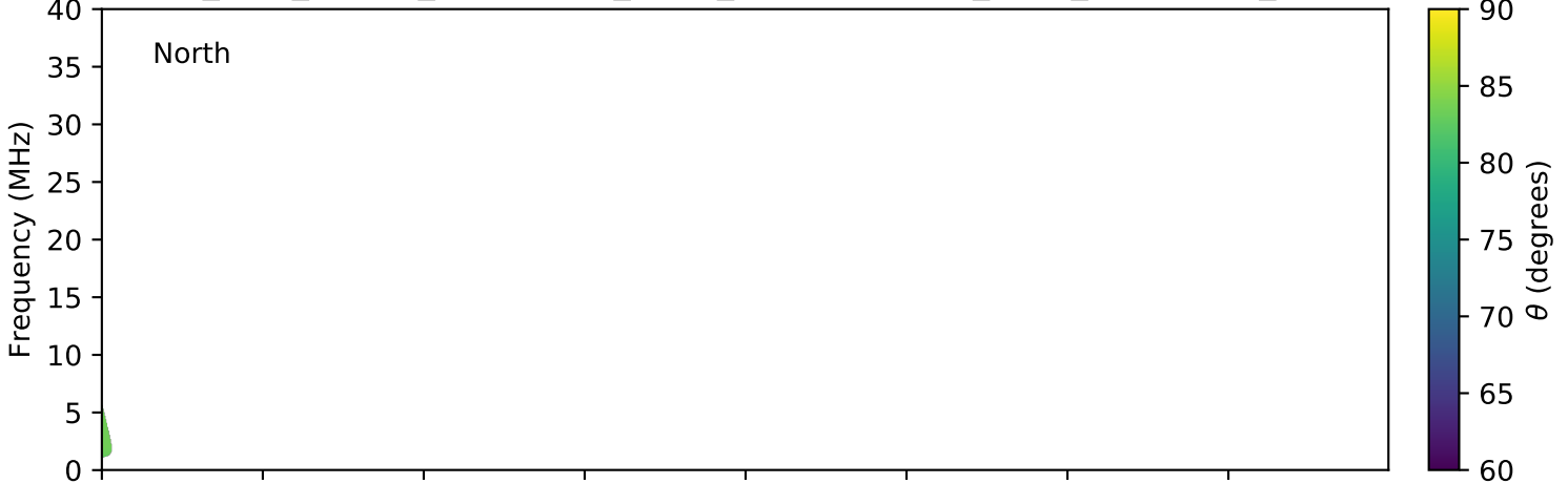
expres_juno_jupiter_ganymede_isaac_lossc-wid1deg_3kev_20170814_v01.cdf
