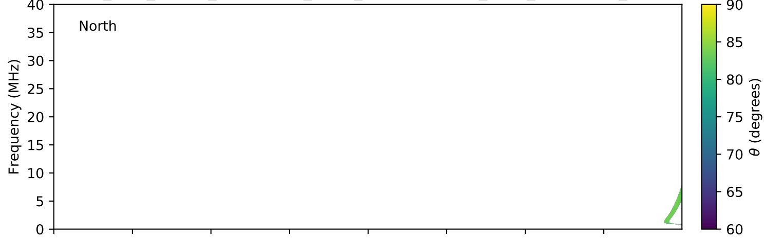
expres_juno_jupiter_ganymede_isaac_lossc-wid1deg_3kev_20170810_v01.cdf
