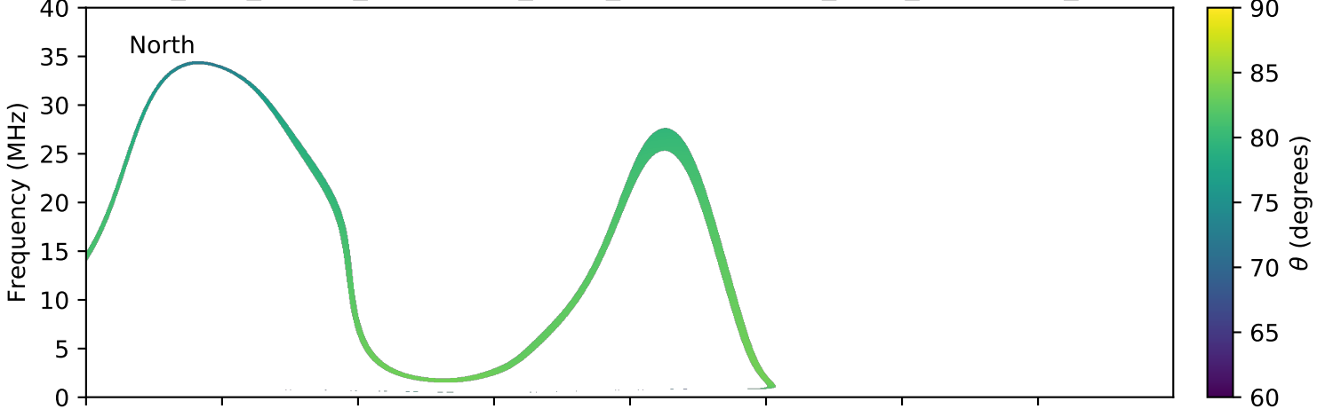
expres_juno_jupiter_ganymede_isaac_lossc-wid1deg_3kev_20170806_v01.cdf
