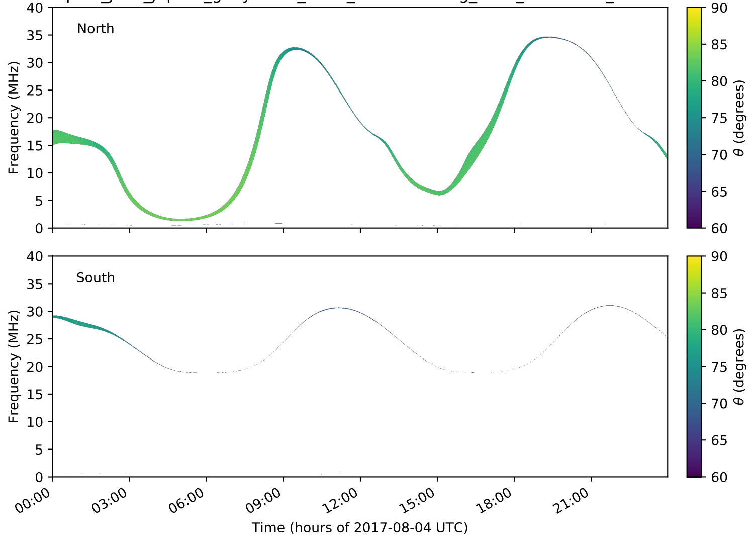
expres_juno_jupiter_ganymede_isaac_lossc-wid1deg_3kev_20170804_v01.cdf
