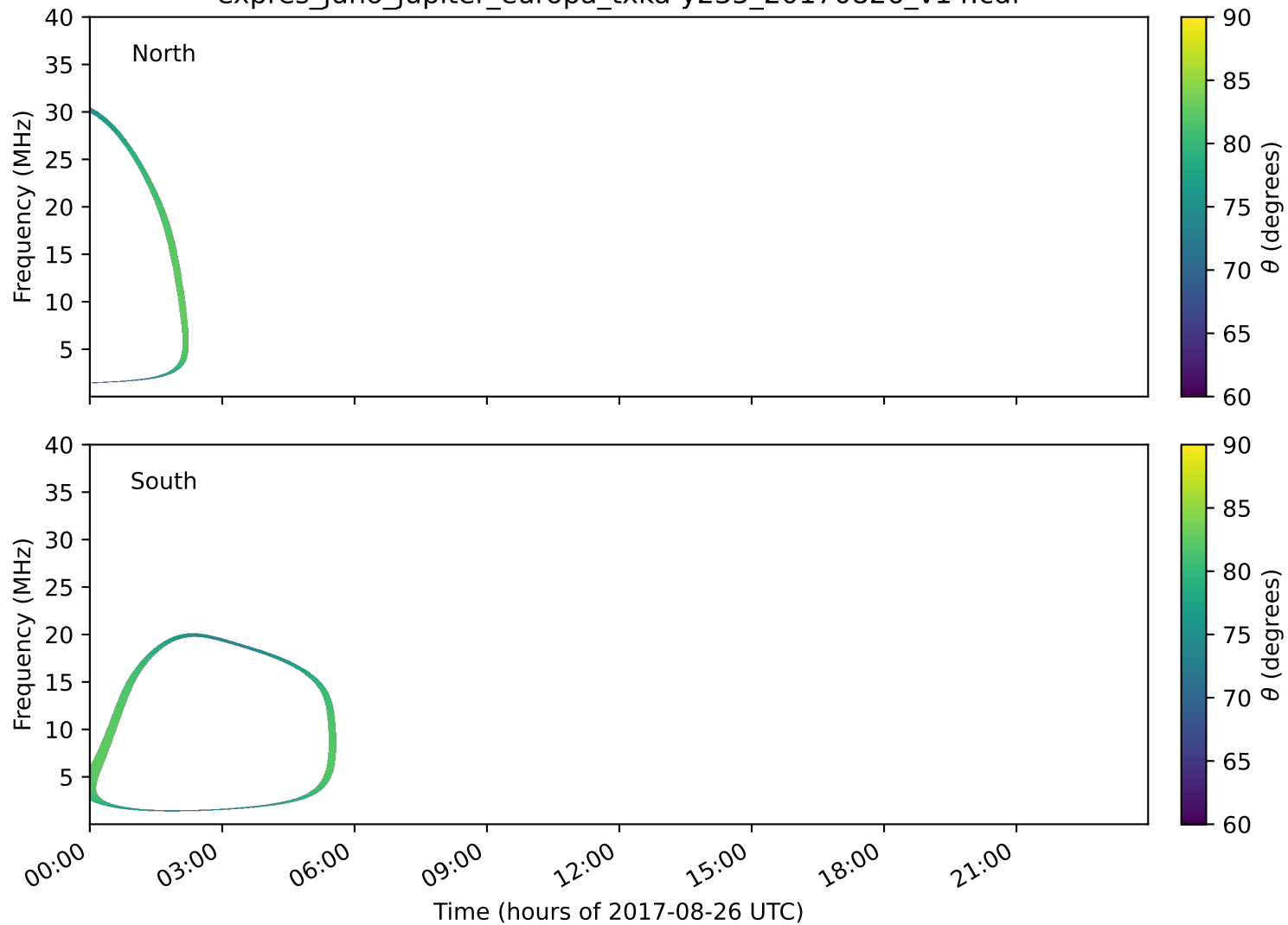
expres_juno_jupiter_europa_txka-y235_20170826_v14.cdf
