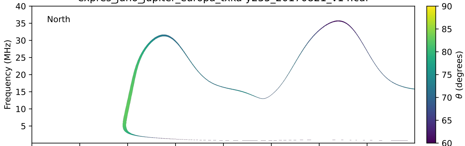
expres_juno_jupiter_europa_txka-y235_20170821_v14.cdf
