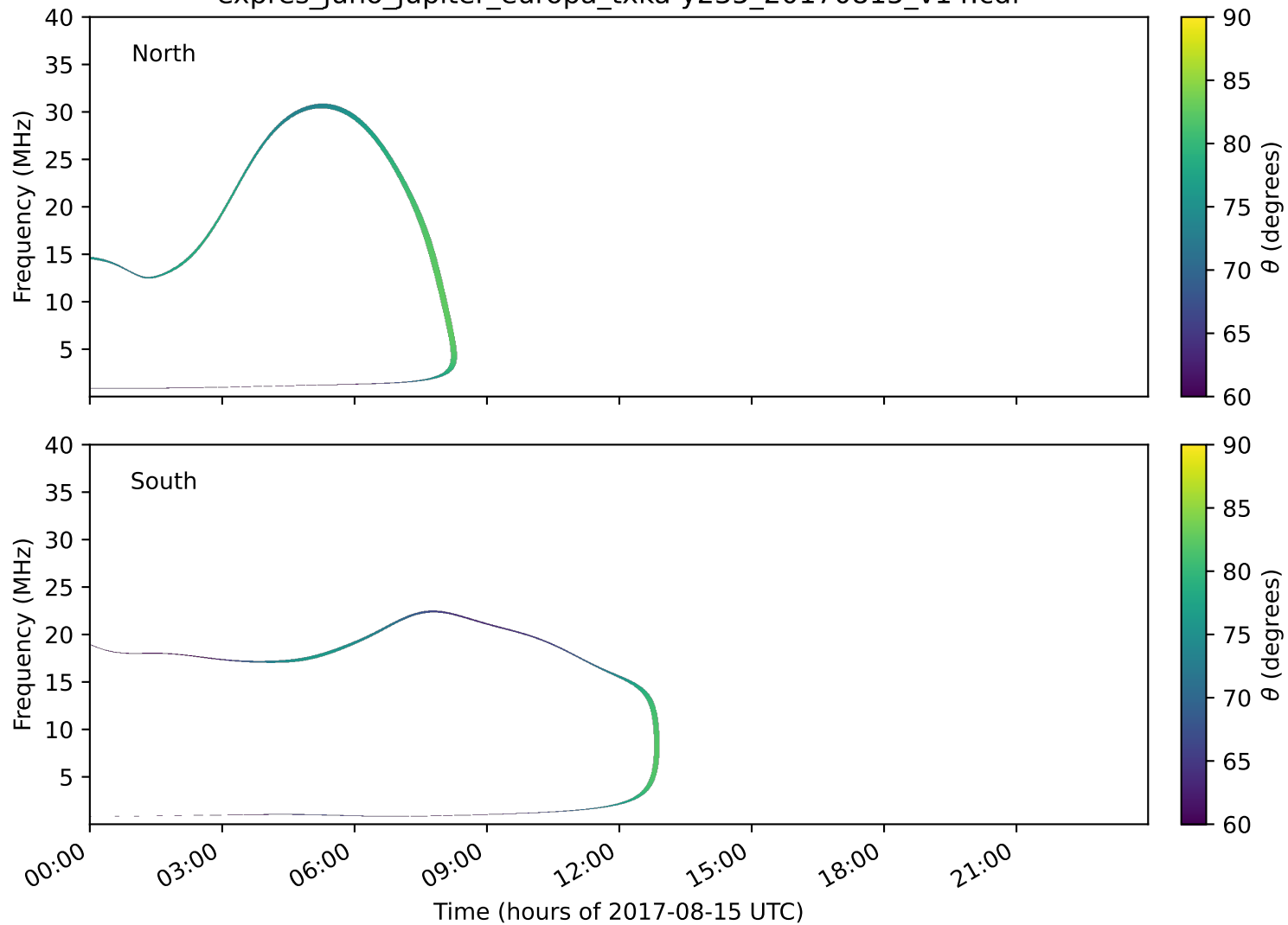
expres_juno_jupiter_europa_txka-y235_20170815_v14.cdf
