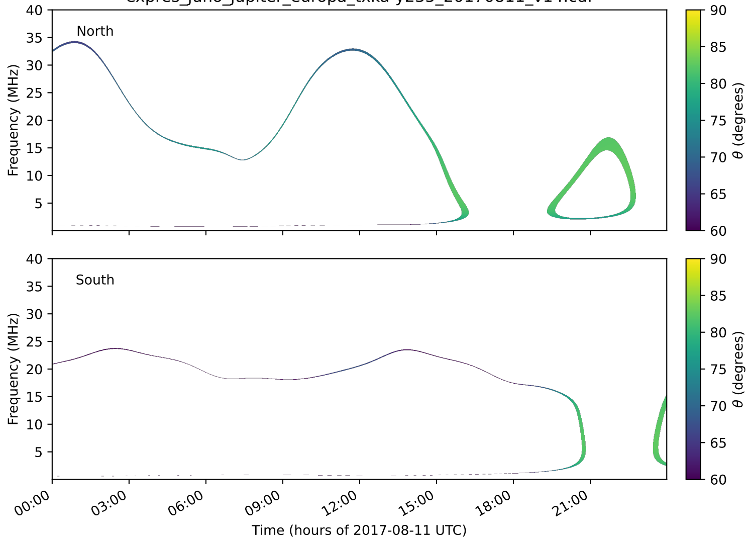
expres_juno_jupiter_europa_txka-y235_20170811_v14.cdf
