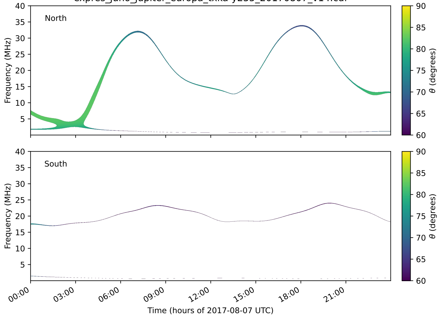
expres_juno_jupiter_europa_txka-y235_20170807_v14.cdf
