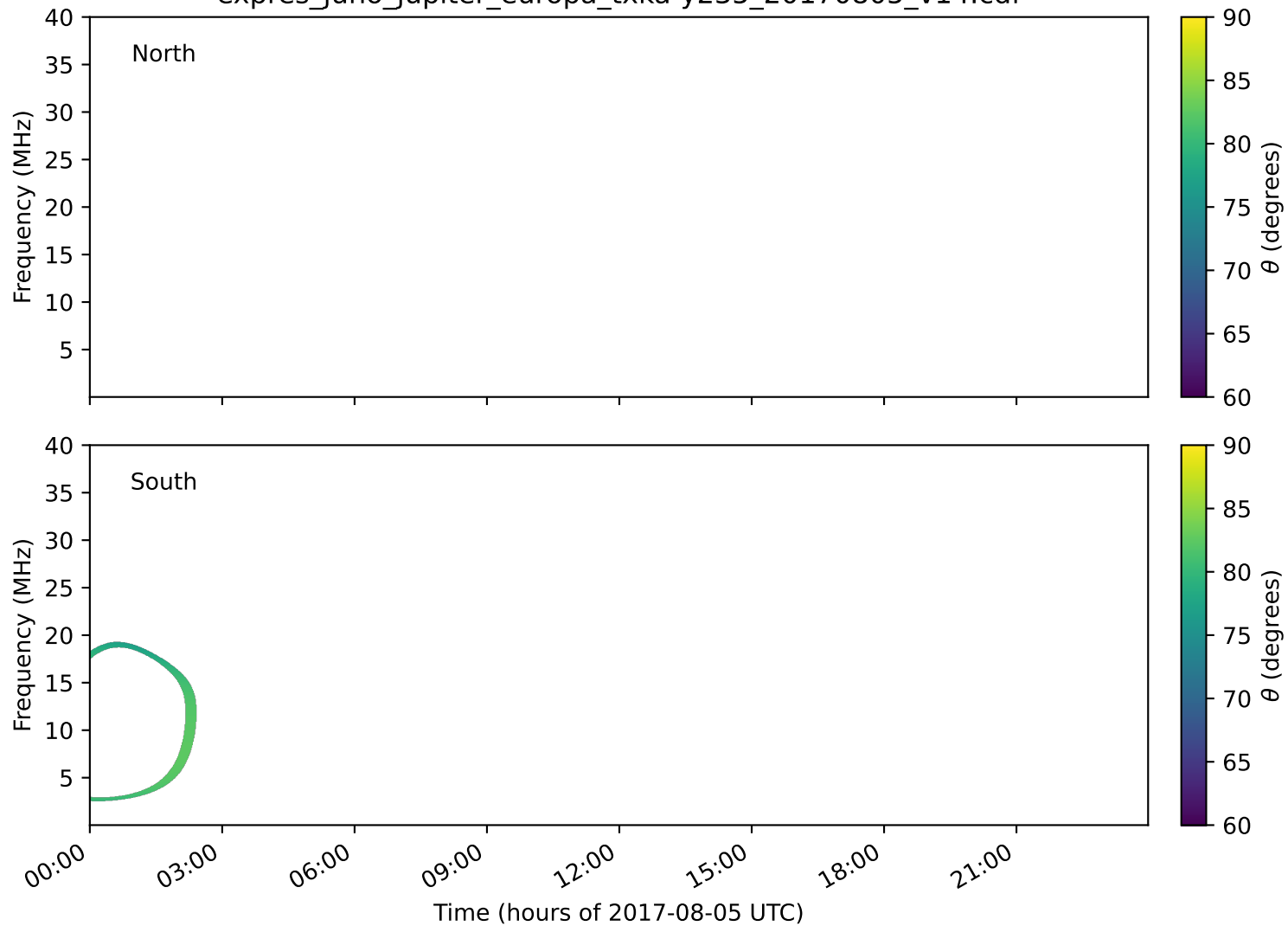
expres_juno_jupiter_europa_txka-y235_20170805_v14.cdf
