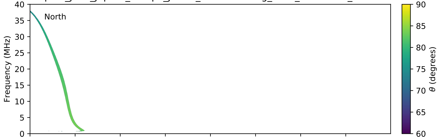
expres_juno_jupiter_europa_jrm09_lossc-wid1deg_3kev_20170826_v01.cdf
