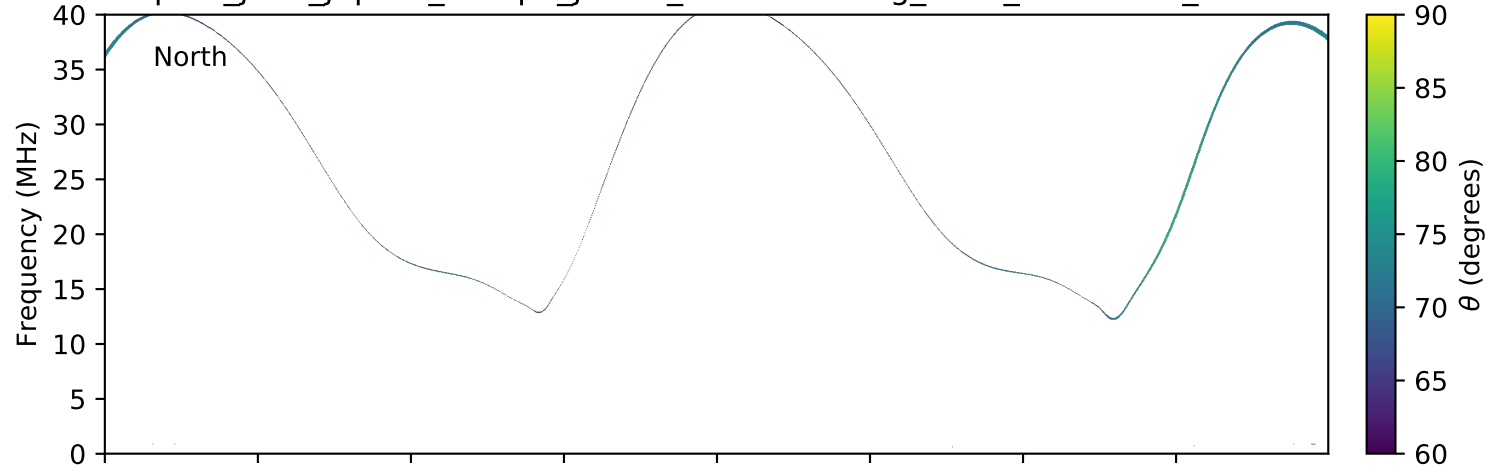
expres_juno_jupiter_europa_jrm09_lossc-wid1deg_3kev_20170825_v01.cdf
