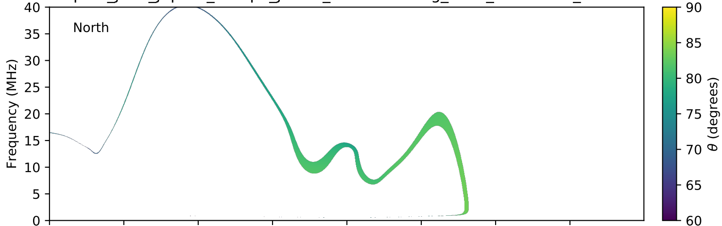
expres_juno_jupiter_europa_jrm09_lossc-wid1deg_3kev_20170822_v01.cdf
