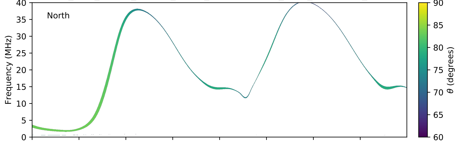
expres_juno_jupiter_europa_jrm09_lossc-wid1deg_3kev_20170807_v01.cdf
