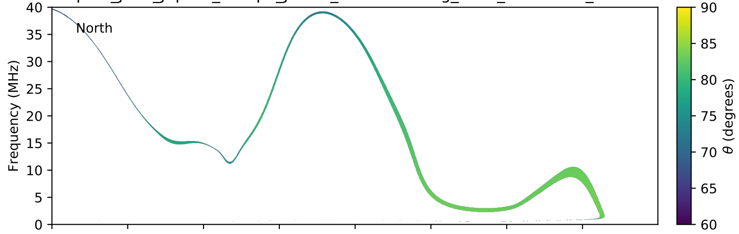
expres_juno_jupiter_europa_jrm09_lossc-wid1deg_3kev_20170804_v01.cdf
