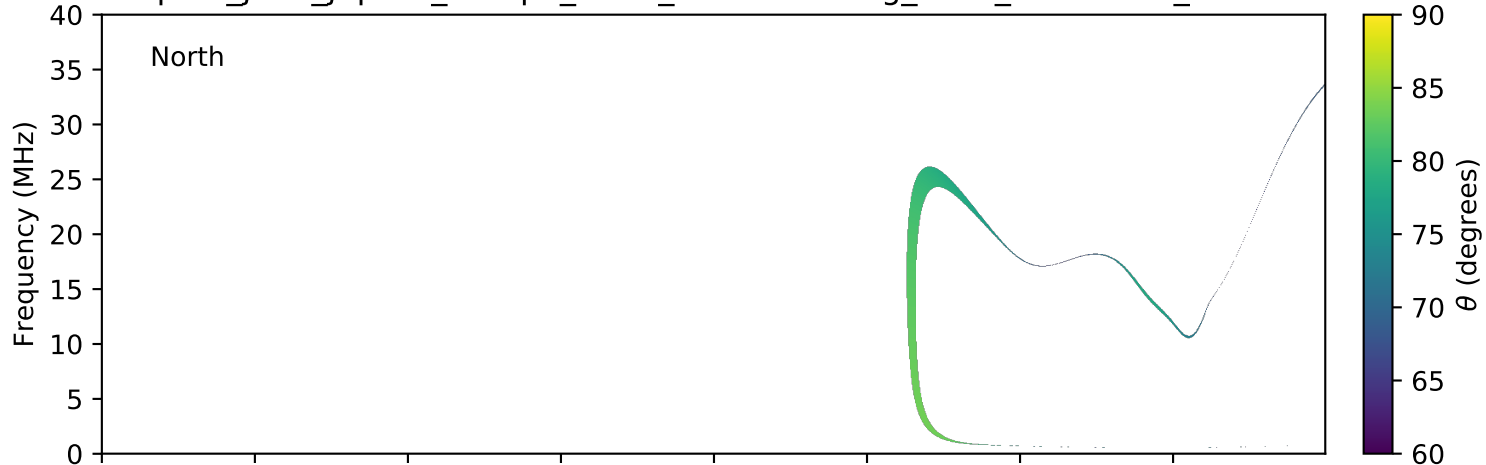
expres_juno_jupiter_europa_isaac_lossc-wid1deg_3kev_20170831_v01.cdf
