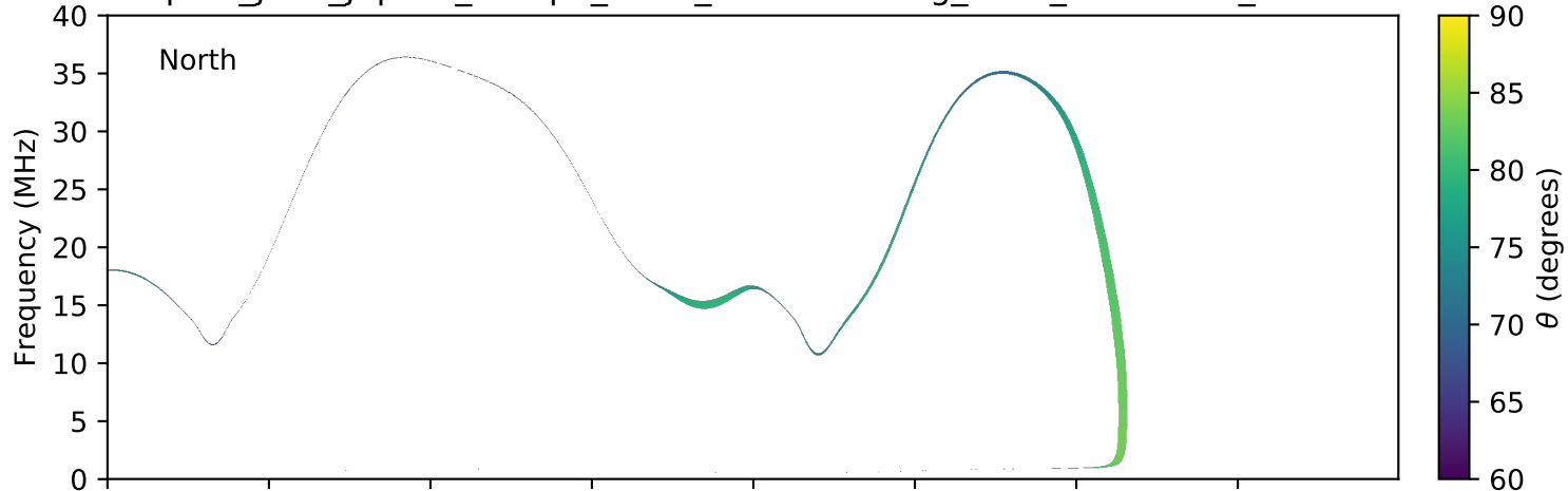
expres_juno_jupiter_europa_isaac_lossc-wid1deg_3kev_20170829_v01.cdf
