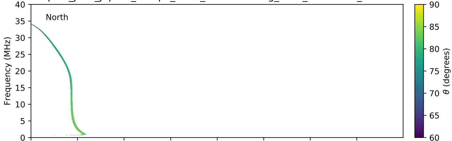
expres_juno_jupiter_europa_isaac_lossc-wid1deg_3kev_20170826_v01.cdf
