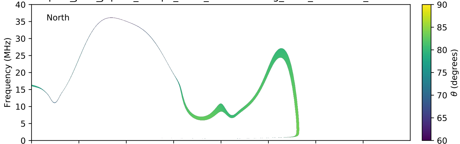
expres_juno_jupiter_europa_isaac_lossc-wid1deg_3kev_20170822_v01.cdf
