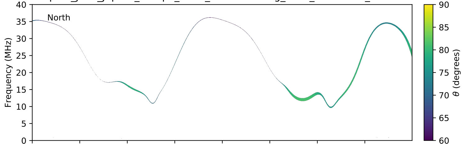
expres_juno_jupiter_europa_isaac_lossc-wid1deg_3kev_20170818_v01.cdf
