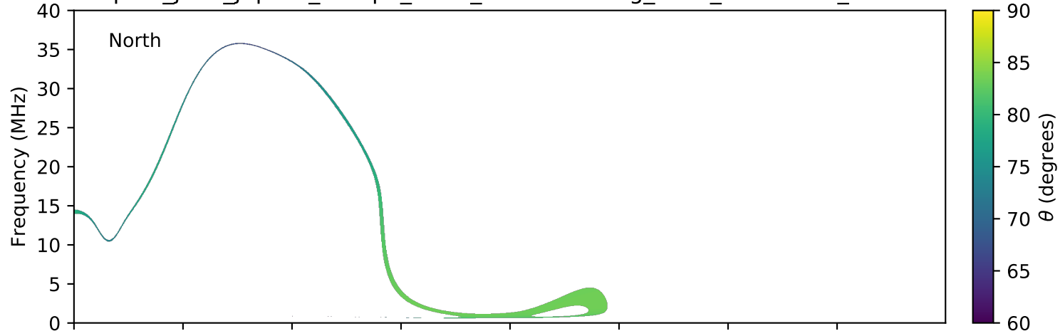
expres_juno_jupiter_europa_isaac_lossc-wid1deg_3kev_20170815_v01.cdf
