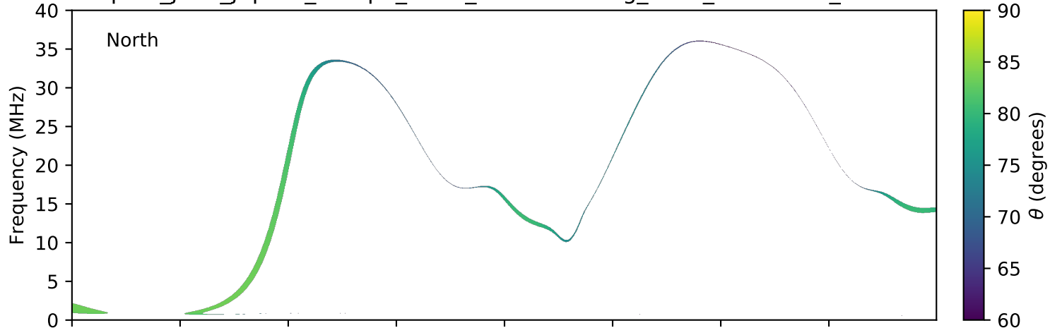
expres_juno_jupiter_europa_isaac_lossc-wid1deg_3kev_20170814_v01.cdf
