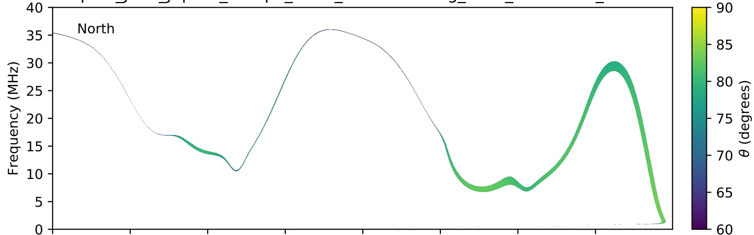
expres_juno_jupiter_europa_isaac_lossc-wid1deg_3kev_20170811_v01.cdf
