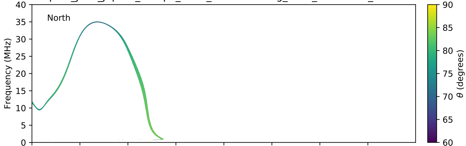
expres_juno_jupiter_europa_isaac_lossc-wid1deg_3kev_20170808_v01.cdf
