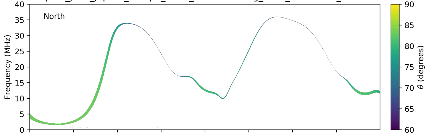
expres_juno_jupiter_europa_isaac_lossc-wid1deg_3kev_20170807_v01.cdf
