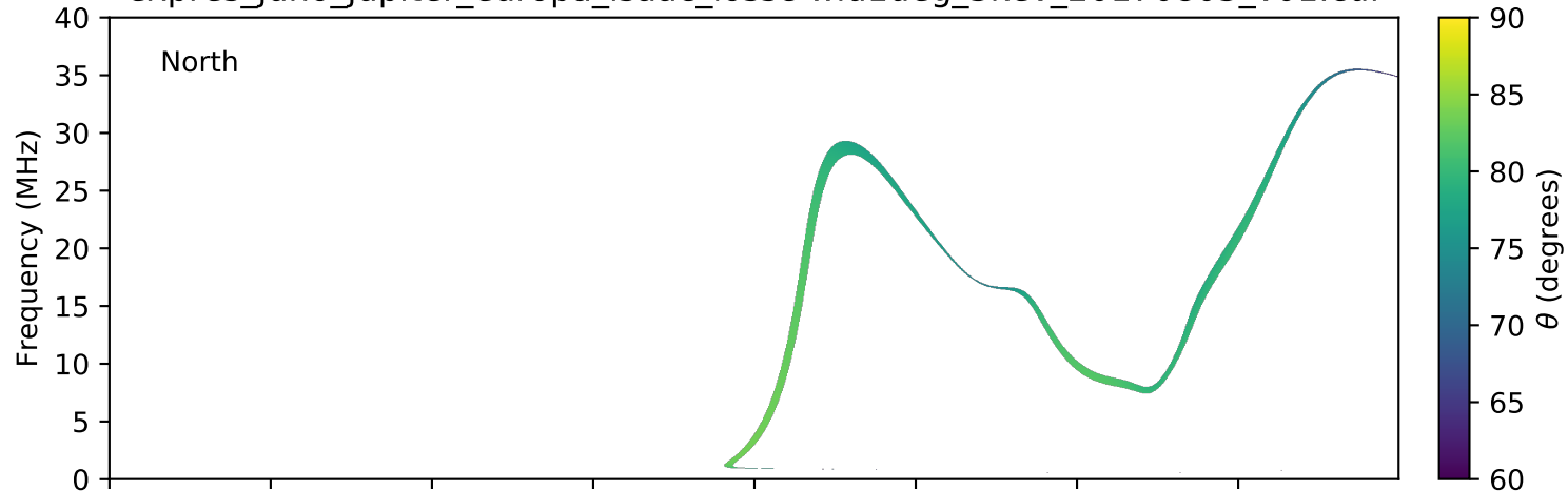
expres_juno_jupiter_europa_isaac_lossc-wid1deg_3kev_20170803_v01.cdf
