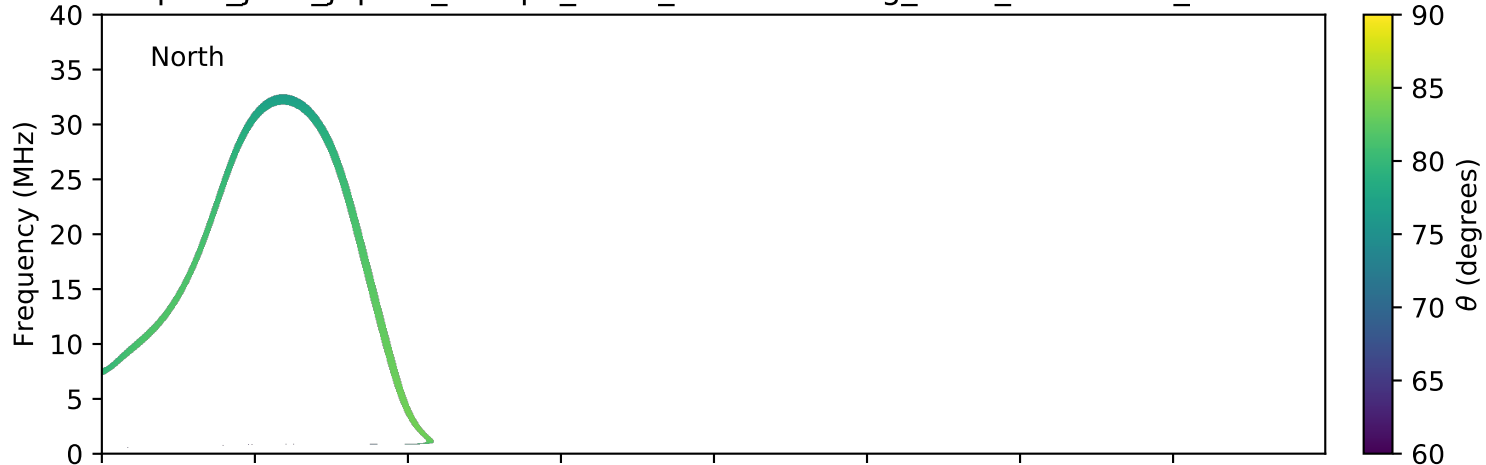
expres_juno_jupiter_europa_isaac_lossc-wid1deg_3kev_20170801_v01.cdf
