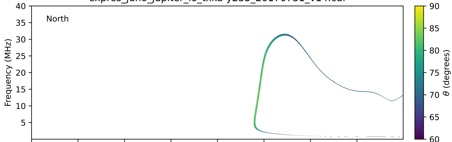
expres_juno_jupiter_io_txka-y235_20170731_v14.cdf
