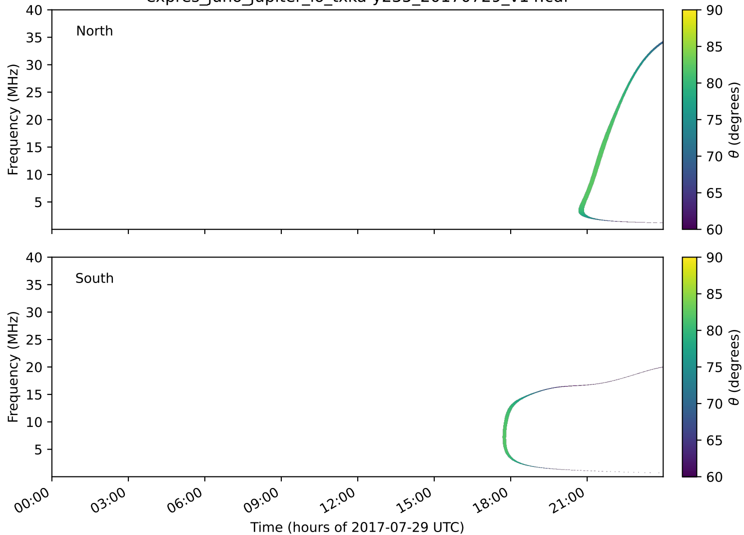
expres_juno_jupiter_io_txka-y235_20170729_v14.cdf
