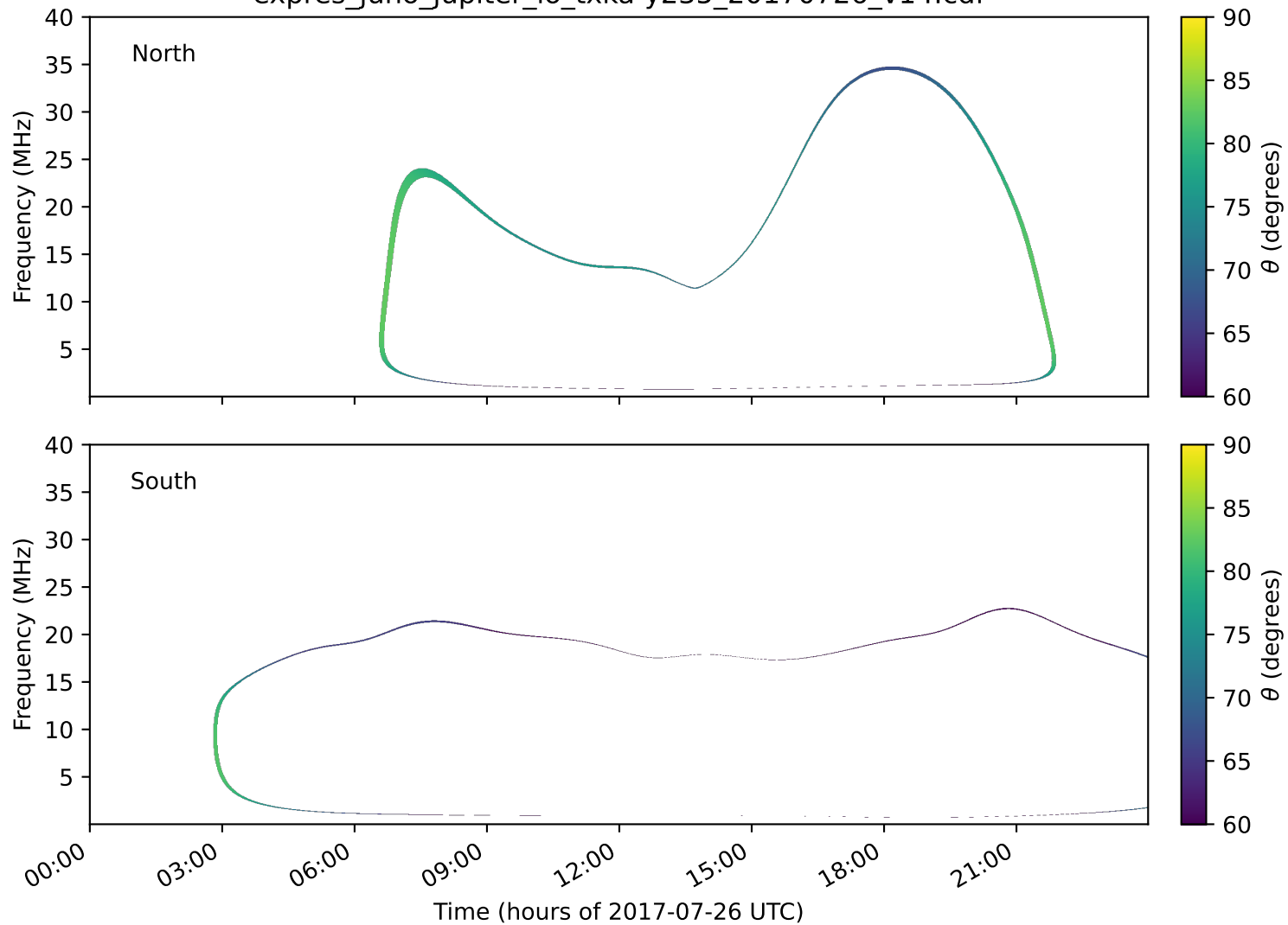
expres_juno_jupiter_io_txka-y235_20170726_v14.cdf
