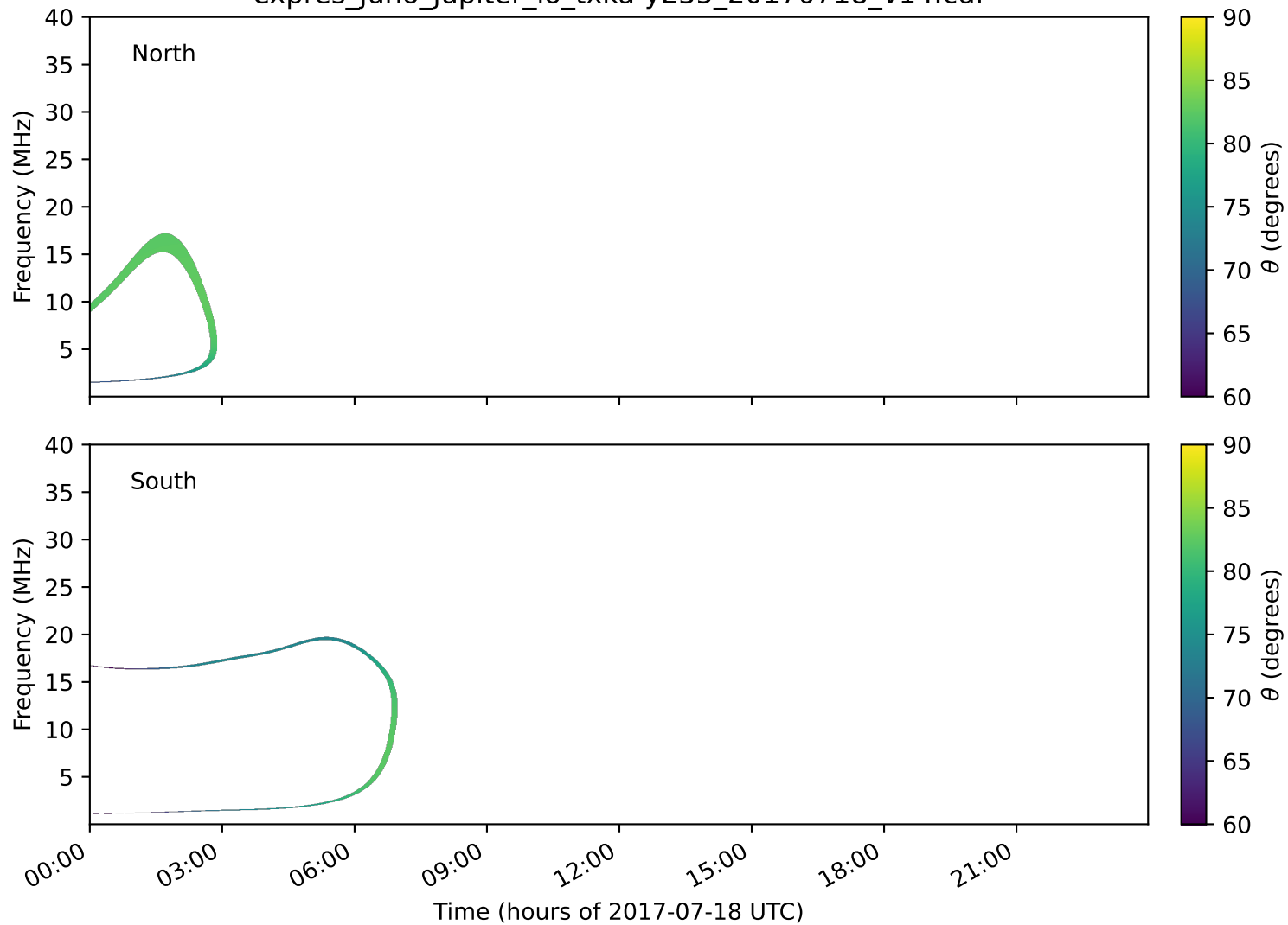
expres_juno_jupiter_io_txka-y235_20170718_v14.cdf
