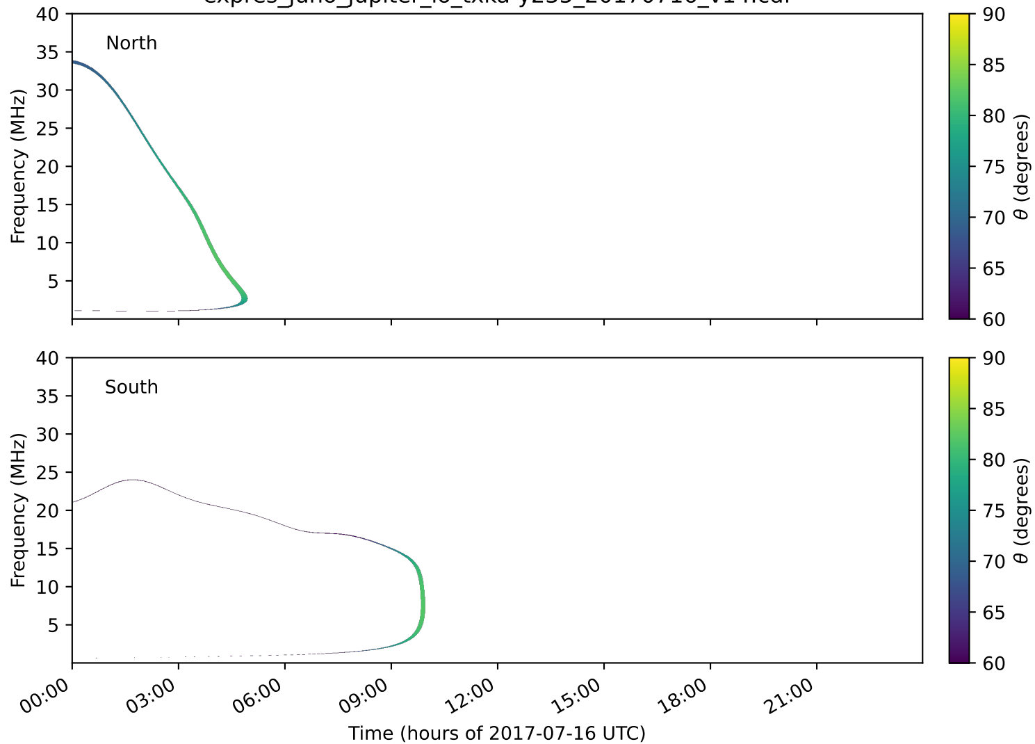
expres_juno_jupiter_io_txka-y235_20170716_v14.cdf
