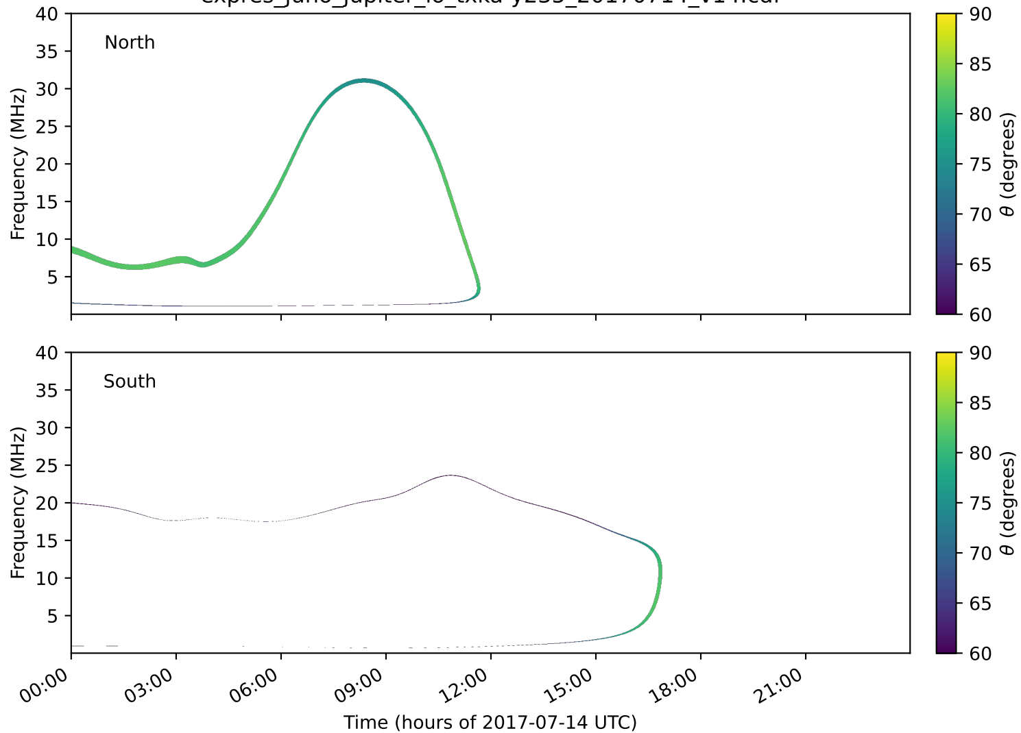
expres_juno_jupiter_io_txka-y235_20170714_v14.cdf
