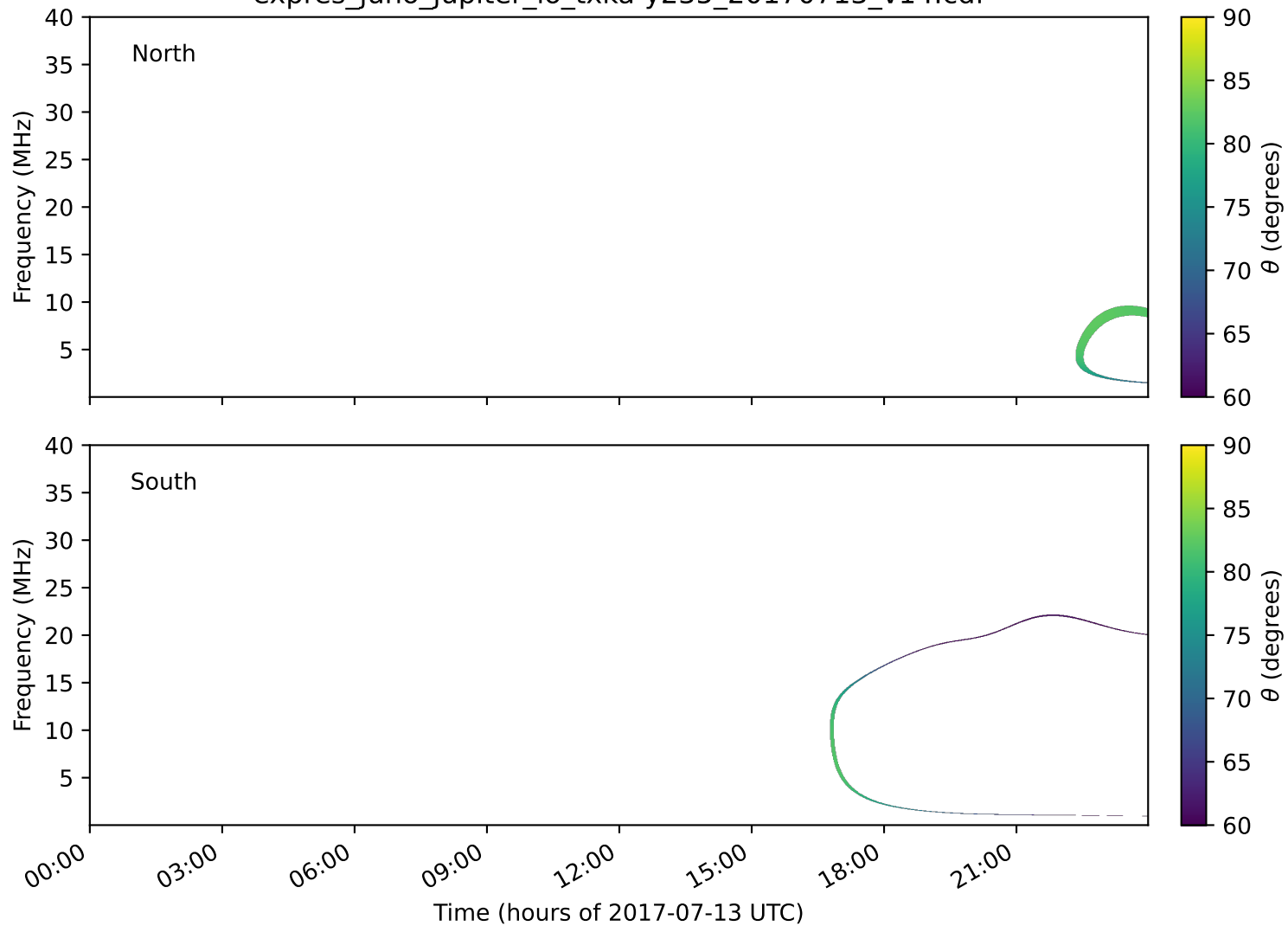
expres_juno_jupiter_io_txka-y235_20170713_v14.cdf
