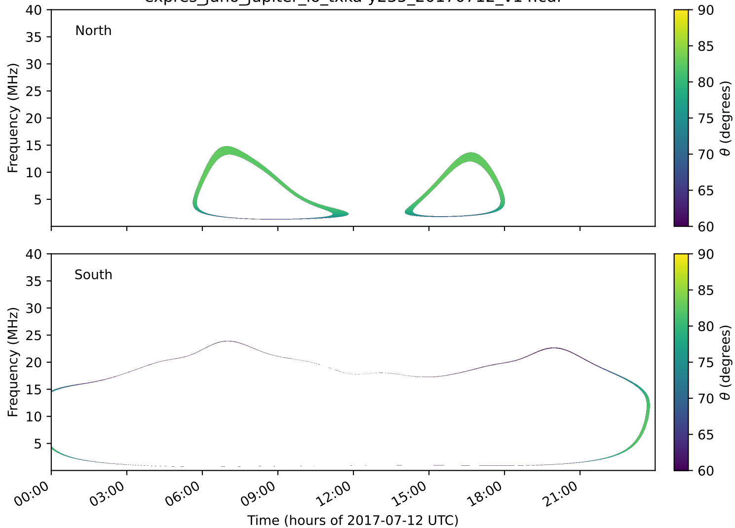
expres_juno_jupiter_io_txka-y235_20170712_v14.cdf
