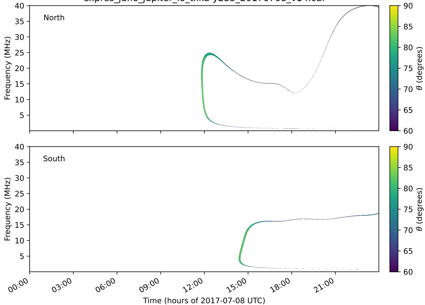
expres_juno_jupiter_io_txka-y235_20170708_v14.cdf
