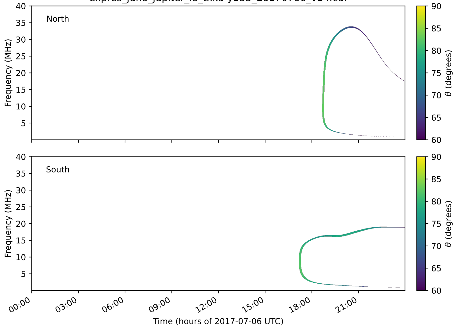
expres_juno_jupiter_io_txka-y235_20170706_v14.cdf
