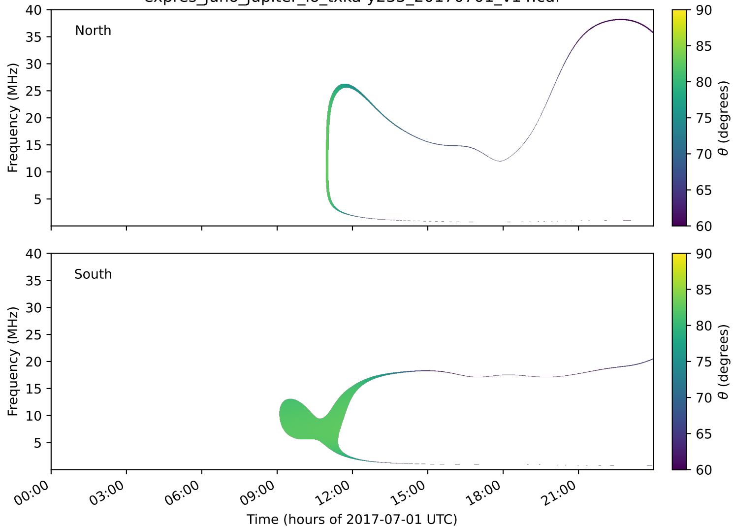
expres_juno_jupiter_io_txka-y235_20170701_v14.cdf
