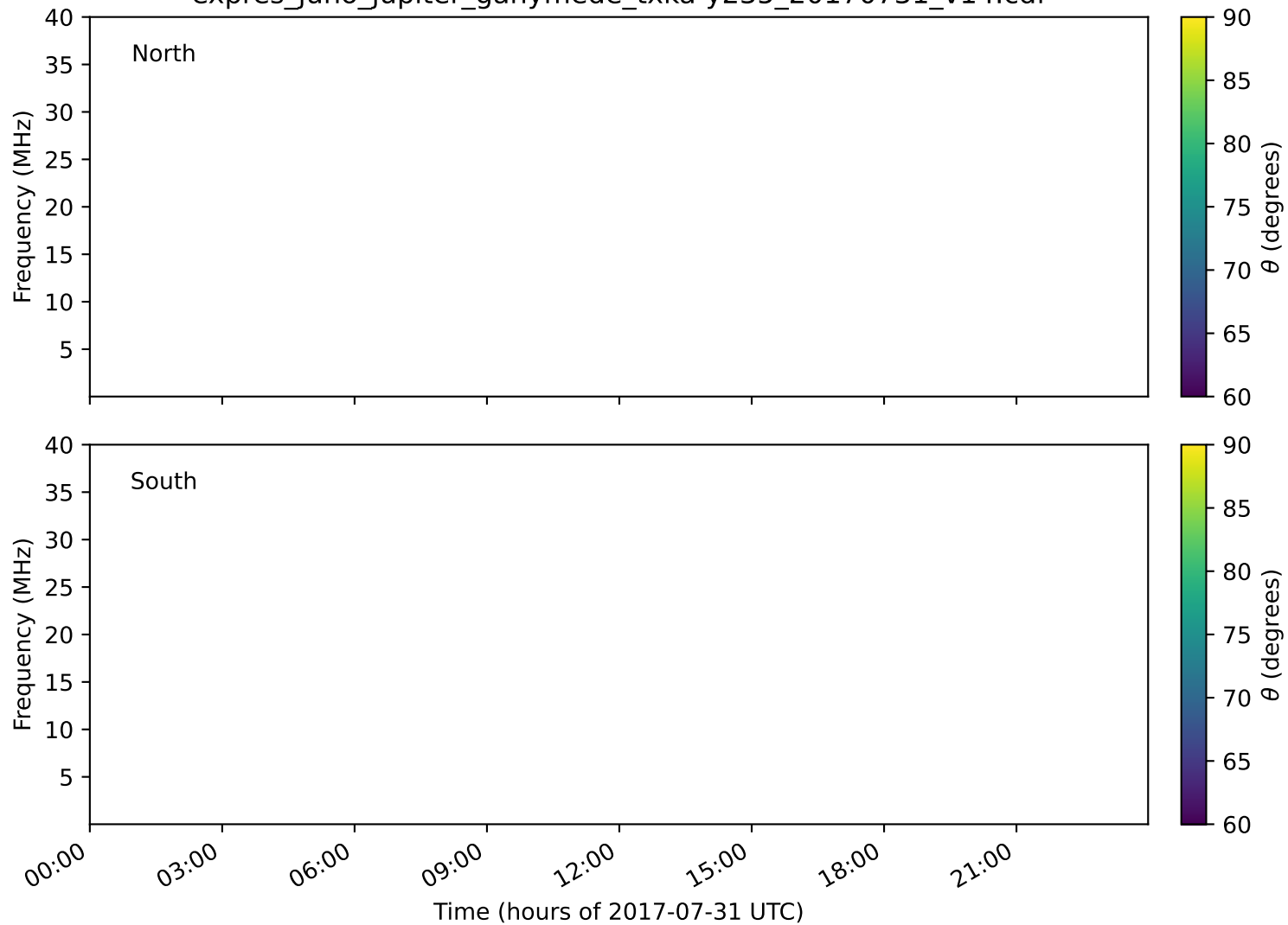
expres_juno_jupiter_ganymede_txka-y235_20170731_v14.cdf
