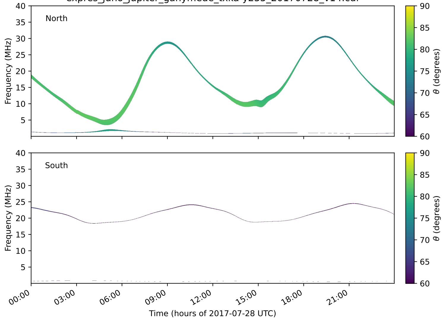
expres_juno_jupiter_ganymede_txka-y235_20170728_v14.cdf
