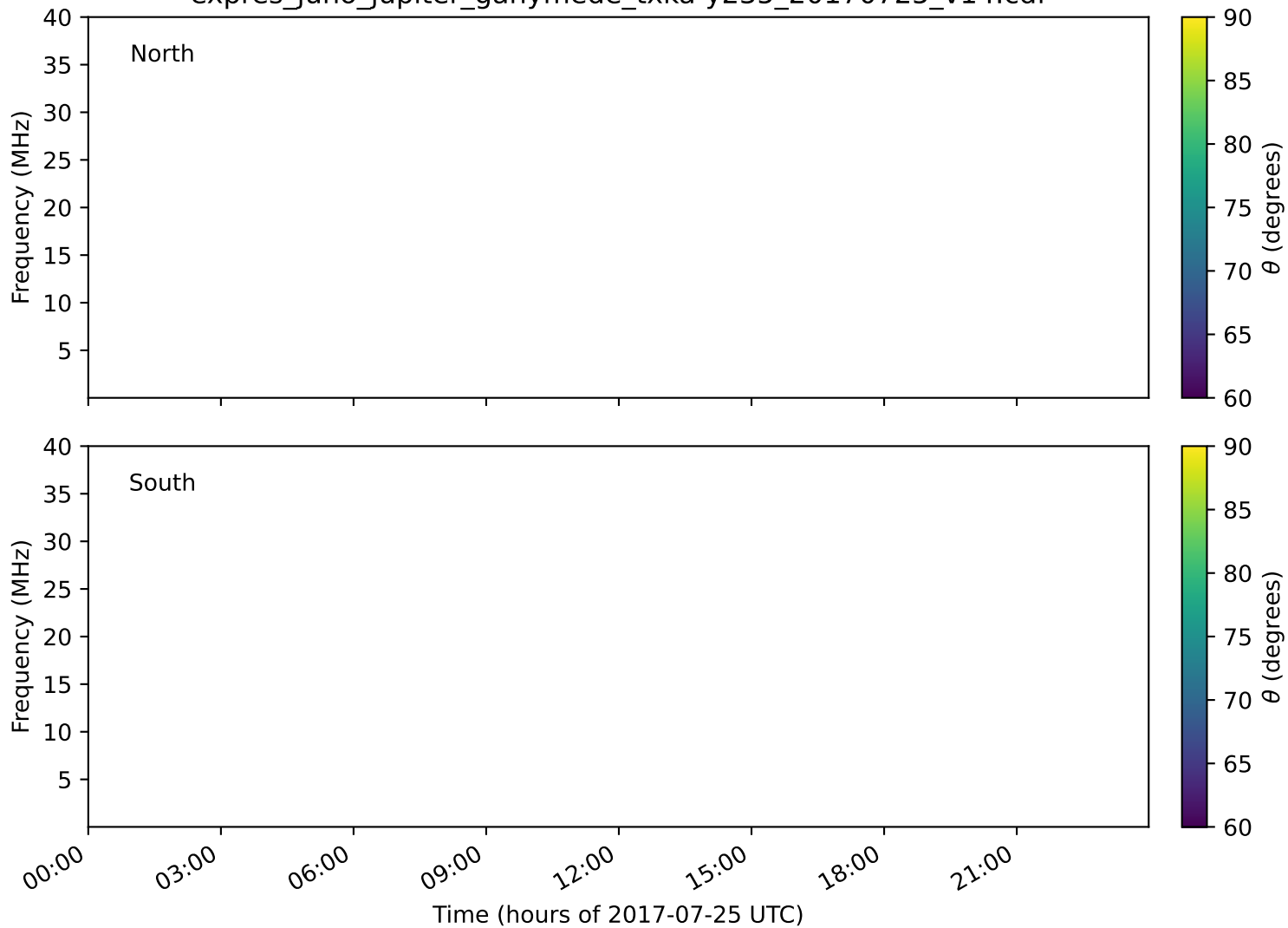
expres_juno_jupiter_ganymede_txka-y235_20170725_v14.cdf
