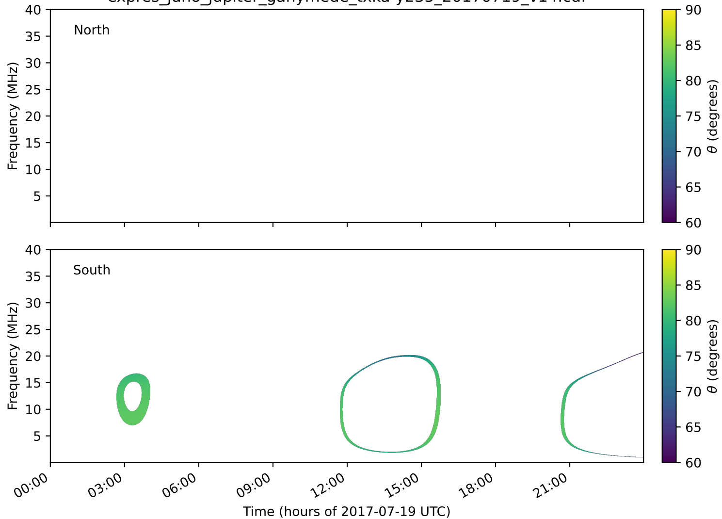
expres_juno_jupiter_ganymede_txka-y235_20170719_v14.cdf
