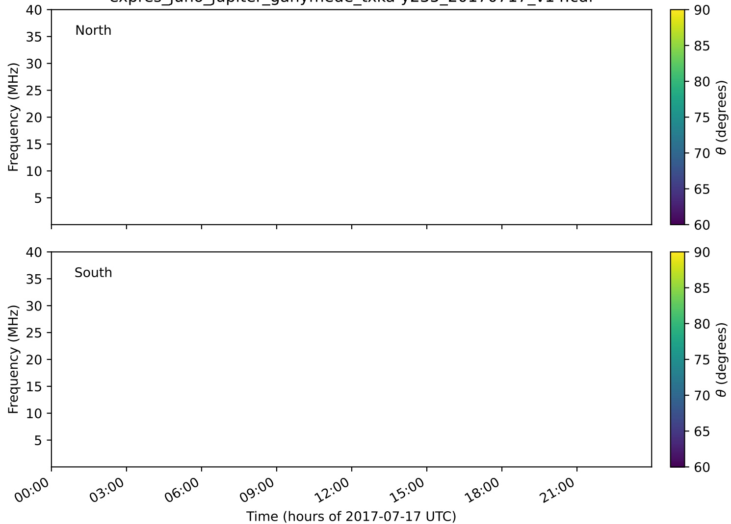
expres_juno_jupiter_ganymede_txka-y235_20170717_v14.cdf
